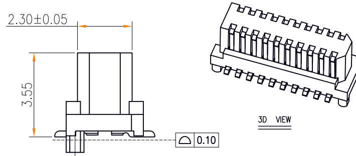
MATING HEIGHT SCALE:1.25:1
