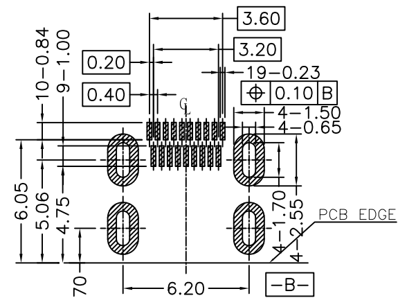
RECOMMENDED PCB LAYOUT(.XX±0.05) CONNECTOR SIDE(TOP VIEW)
