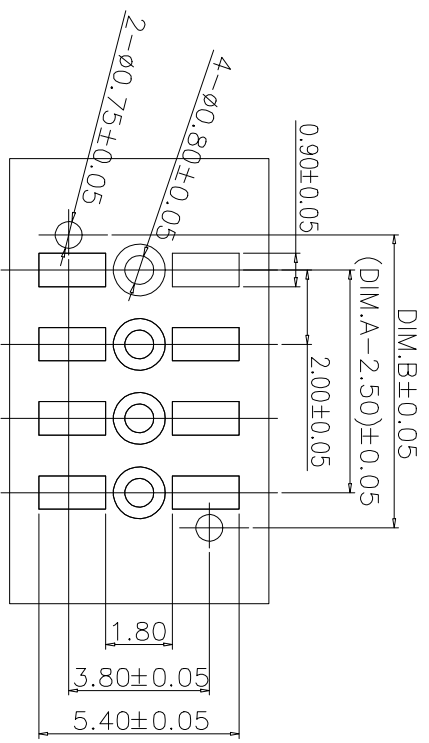
P.C.B LAYOUT TOLERANCE: ±0.05
